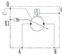
Hydraulic Diagram
